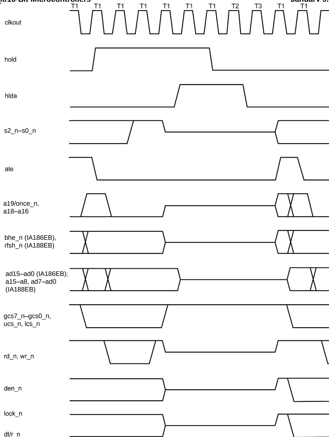
Figure 24. hold/hlda Timing
