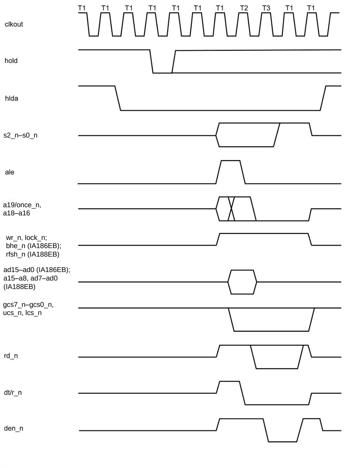
Figure 25. Refresh During Hold Acknowledge Timing
